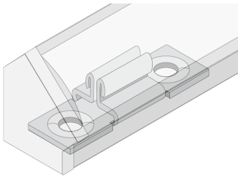
Chromapath Surface Mount Total Dimensions: 0.61 × 0.82 (H x W)
